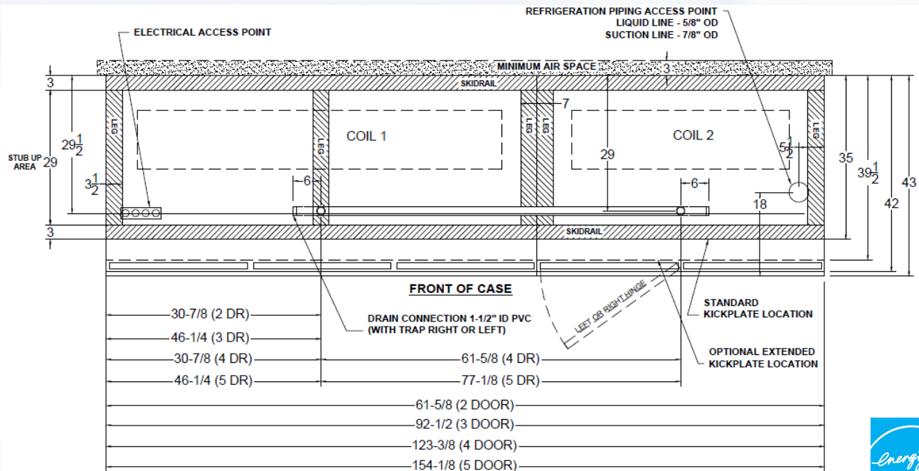
RX7SL Plan View
