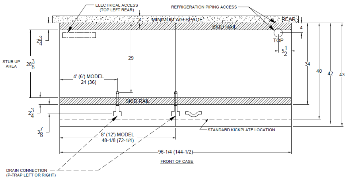
DX6UD PLAN VIEW (SINGLE COIL)
